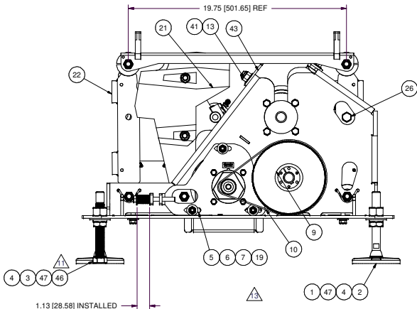
SECTION A-A SCALE 1 / 4
